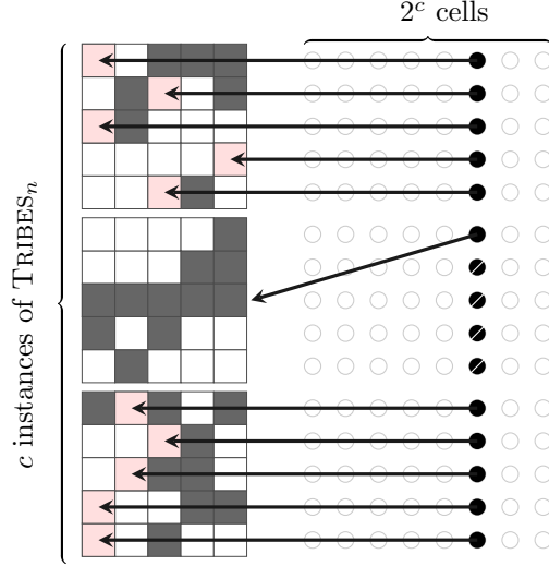
Figure 1: Function f := (\text{TRIBES}_n)_{\text{CS}} . The 1-entries of the n -by- n matrices x_j are drawn as white, and the 0-entries are drawn as black. The arrows illustrate the pointers encoded inside a single cell C_\ell that certifies \text{TRIBES}_n(x_1) = 1 , \text{TRIBES}_n(x_2) = 0 , and \text{TRIBES}_n(x_3) = 1 .
