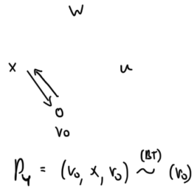
Figure 2: A contraction for an edge uw
