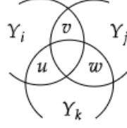
Figure 3: A triangle in X , in \mathcal{A} , and in the GK decomposition
