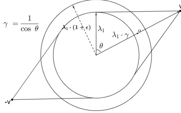
Figure 4: Adversarial Convex Body
