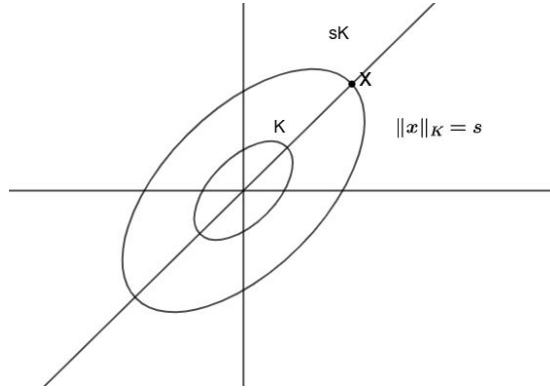
Figure 1: Norm w.r.t. O-symmetric convex body
