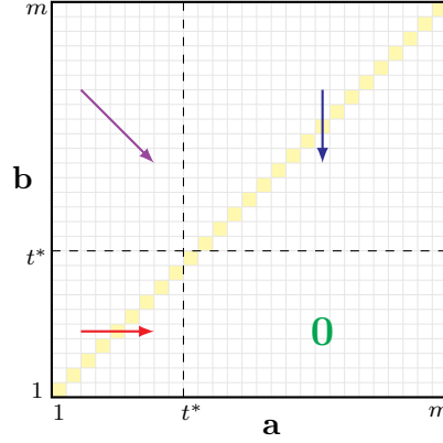
Figure 1: Illustration of updates on the sign coordinates a, b before swapping them, when the translated projections of X and Y are fixed points of G_{H_a} and G_{H_b} . We increase a by one when a < t^* and decrease b by one when b > t^* . Hence, the bottom-left region moves right, the top-right region moves down, the top-left region moves both right and down, and the bottom-right region remains unchanged. The yellow cells mark the diagonal a = b , which is fixed under our swapping operation. This illustrates how the update and swap rules single out (t^*, t^*) as the sign coordinates of the unique fixed point of our constructed functions.
