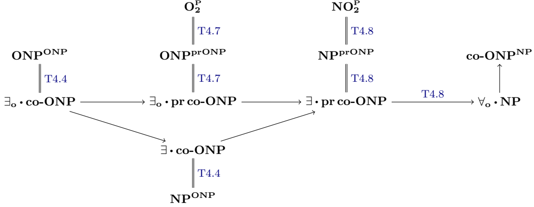
Figure 2: Diagram of equivalences and containments for classes with ONP and prONP oracles
