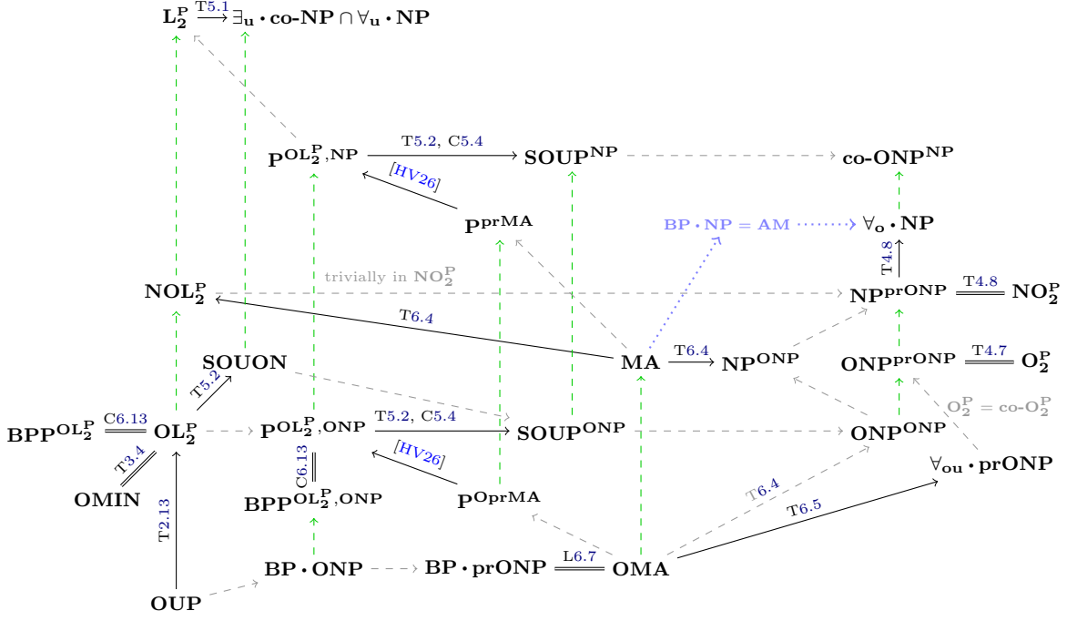
Figure 1: Overview of containments. Legend: solid arrow or equivalence — interesting containment, dashed arrow — this containment is trivial or follows from other results, dotted arrow — not discussed in the paper, shown to give a better perspective. The full version contains more details.
