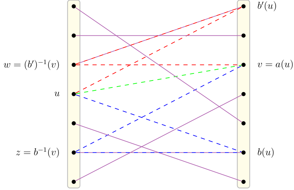
Figure 1: An illustration of the 6-cycle in the proof of Lemma 4.5 , with n = 7 . Red and blue edges correspond to b' and b , respectively. The green edge corresponds to a . Solid purple (=red+blue) edges correspond to \hat{b} = b_{(u,v)} = b'_{(u,v)} . Dashed edges are not included in \hat{b} .
