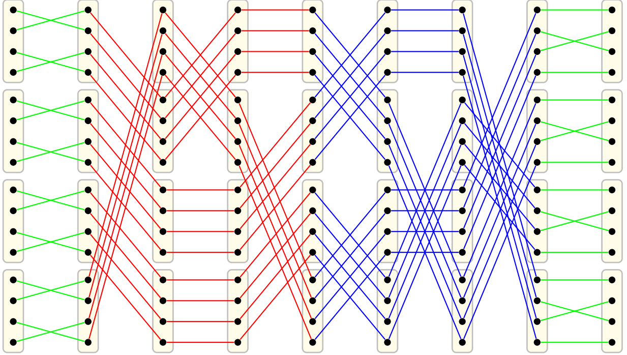
Figure 2: An illustration of the first \ell + 1 layers of permutation and product edges in G , with n = 4, r = 3 and thus \ell = 7 . Each yellow group represents a group of 4 vertices in the same layer. Red edges correspond to permutations A_1 = (1\ 2\ 3\ 4) , A_2 = (1\ 2) , A_3 = (2\ 4\ 3) . Blue edges correspond to inverses of permutations B_1 = (1\ 3\ 2\ 4) , B_2 = (2\ 4) , B_3 = (1\ 2)(3\ 4) in reverse order. Green edges are product edges.
